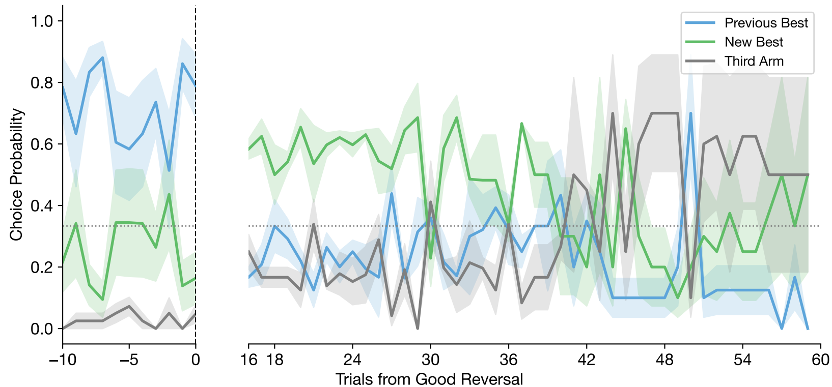
Good Reversal-Aligned Choices (mean \pm se across subjects | n=5 subjects, n=27 reversals) (Skipping first 15 trials post-reversal)
